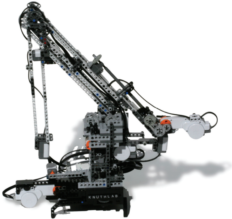
FIGURE 1. A photograph of the robotic arm. The end of the arm is equipped with a light sensor that can make point measurements. The robot is built using the LEGO MINDSTORMS NXT system, and is locally controlled with the NXT brick. The NXT brick can communicate with a laptop computer using Bluetooth. The laptop computer (not shown) runs the inference and inquiry code in MATLAB. At the time of the workshop, the MATLAB to NXT communication was not completely operable, and the system was demonstrated via simulations.
